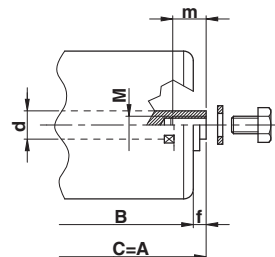
RP asse forato e filettato + vite e rondella (vite UNI 5737) drilled and threaded shaft + bolt and washer (screw UNI 5737)
