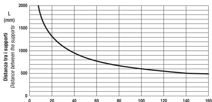
Portata - Load capacity [daN]
